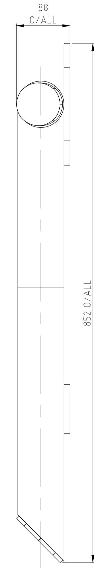
RIGHT VIEW
