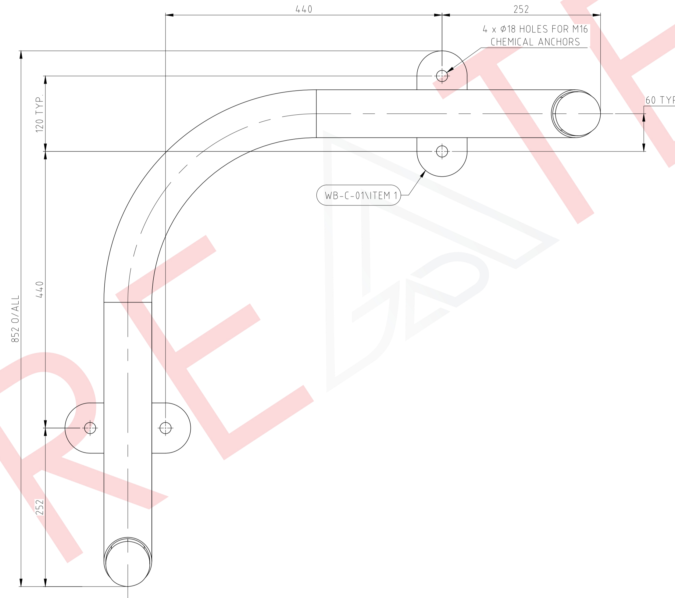
FRONT VIEW WB-C-01
