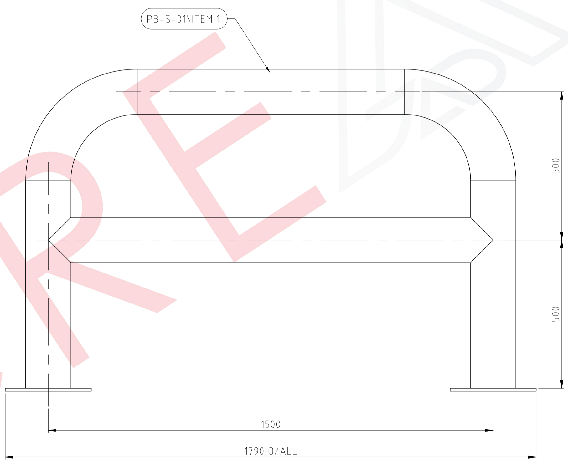
FRONT VIEW PB-S-01
