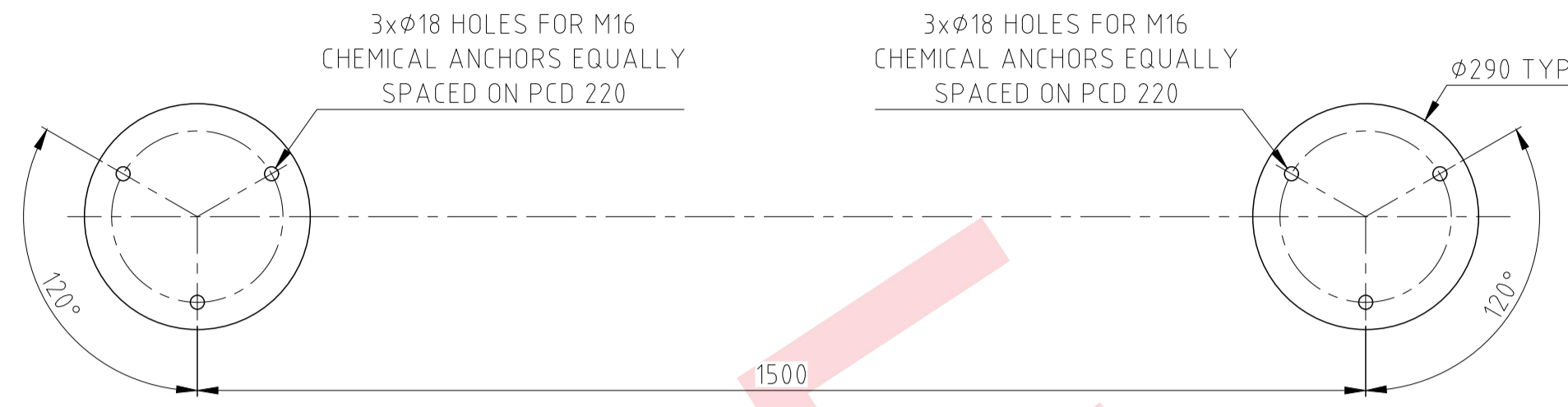
DRILLING DETAIL PB-S-01
