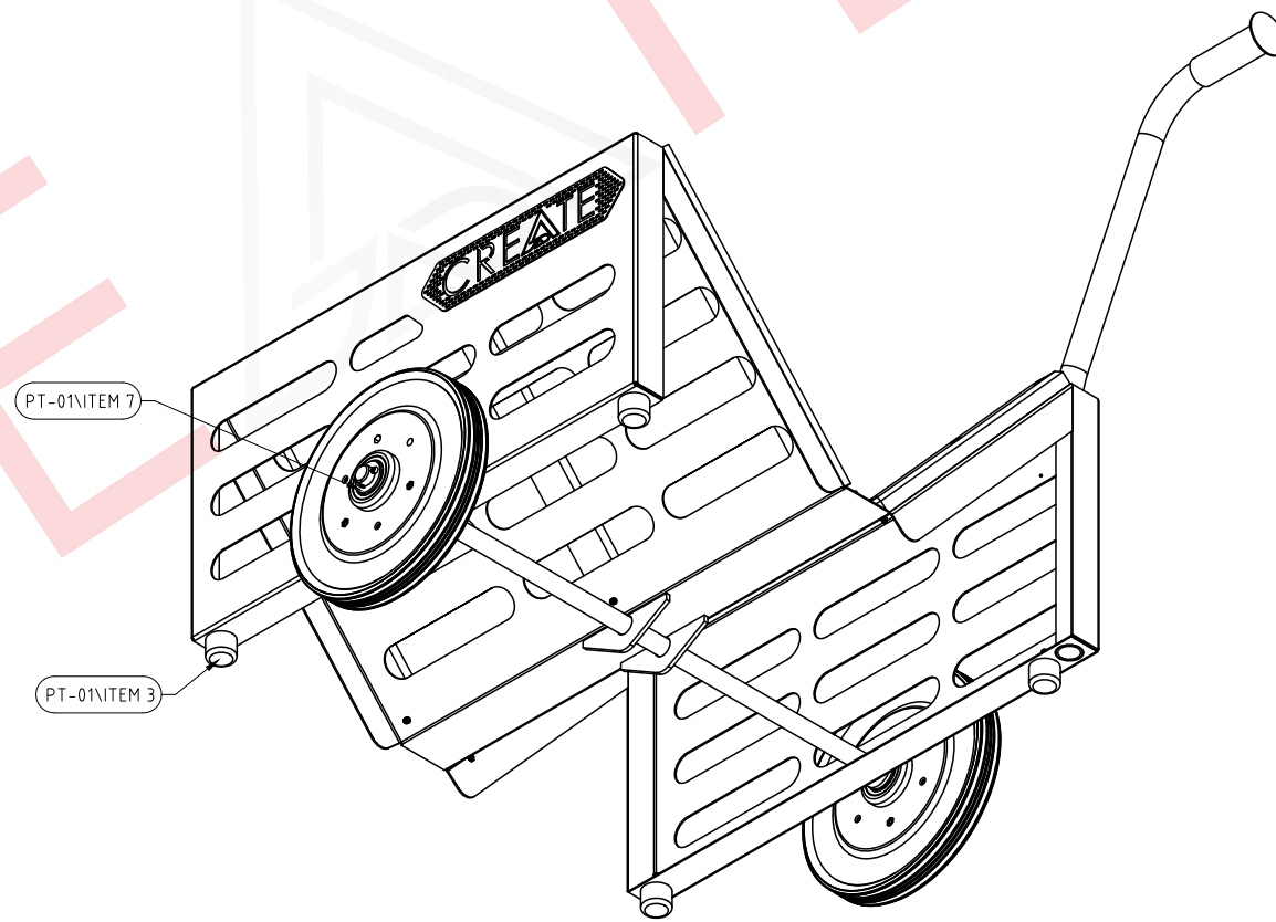
ISOMETRIC VIEW 2 PT-01
