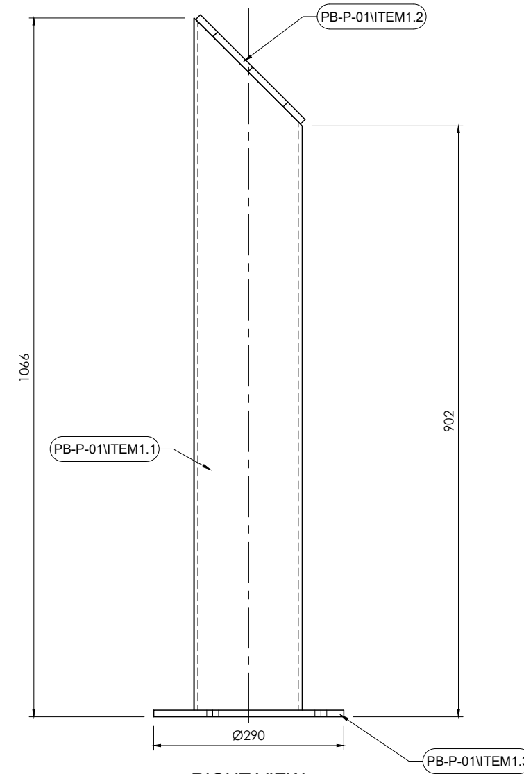
RIGHT VIEW
